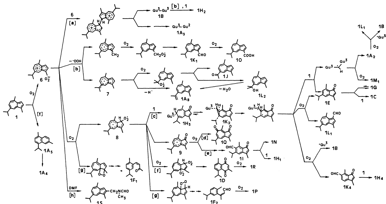
Scheme 1. Possible reaction pathways for the autoxidation products from 1 .
